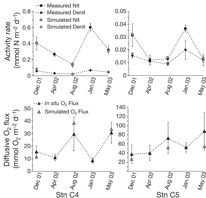
Fig. 3. Comparison of simulated ( \bullet , \blacktriangle , \diamond ) nitrification, denitrification and diffusive oxygen fluxes rates with those calculated from measured in situ oxygen profiles or sediment incubations ( \circ , \triangle , \blacklozenge ) at Stns C4 and C5. In situ nitrification and denitrification rates assessed using the acetylene-blockage method; diffusive oxygen fluxes calculated from in situ microprofiles
