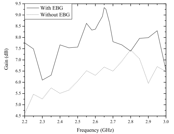
Fig. 10. Measured gain vs. frequency for cylindrical path antennas with classical ground plane or with EBG substrate.
