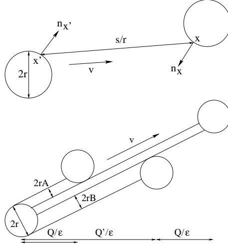
Figure 1. Left: the transfer map (s, h) = T_r(h', v) , with h' = \sin(n_{x'}, v) and h = \sin(n_x, v) . Right: Particles leaving the surface of one obstacle will next collide with one of generically three obstacles. The figure explains the geometrical meaning of A, B, Q .
