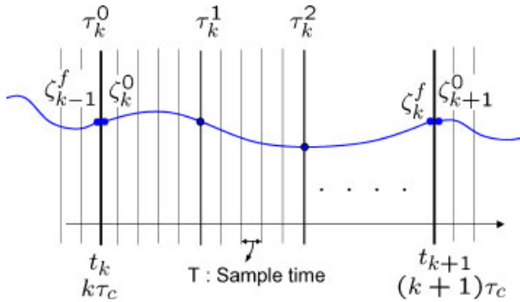
Figure 4. Trajectories illustration.
