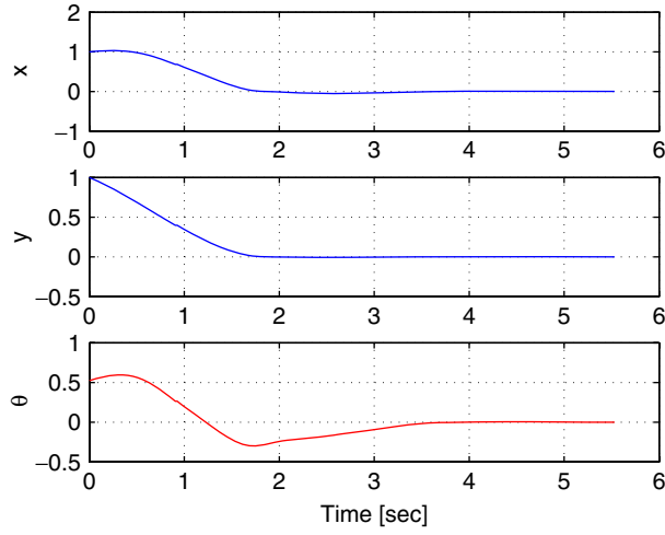
Figure 9. Evolution of the PVTOL position and orientation.
