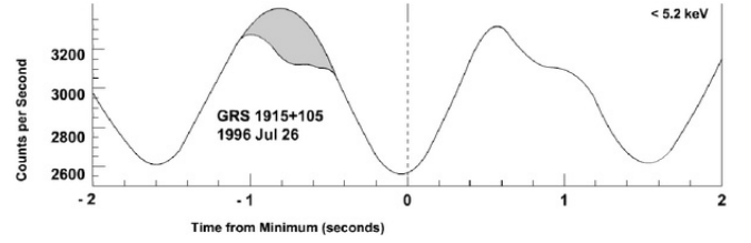
Fig. 1. Morgan et al. (1997) studied GRS 1915 + 105 timing variability using average QPO-folded profile for the 0.63 Hz QPO. The profile shows an absorbed-like feature for the soft energy band (<5.2 keV) emphasized on the figure by the grey “missing part”. Morgan et al. (1997) also showed the QPO profile at higher (hard) energies. For higher energies, the profiles appear more sinusoidal, i.e. the “missing/absorb part” becomes smaller.
