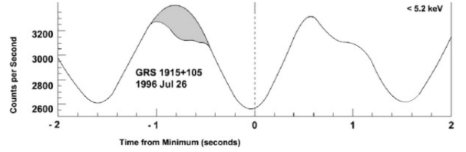
Fig. 1. Morgan et al. (1997) studied GRS 1915 + 105 timing variability using average QPO-folded profile for the 0.63 Hz QPO. The profile shows an absorbed-like feature for the soft energy band (<5.2 keV) emphasized on the figure by the grey “missing part”. Morgan et al. (1997) also showed the QPO profile at higher (hard) energies. For higher energies, the profiles appear more sinusoidal, i.e. the “missing/absorb part” becomes smaller.
