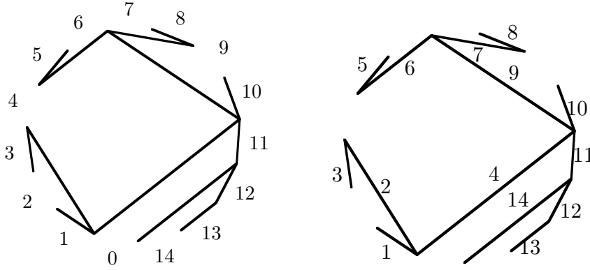
FIGURE 1. A non-crossing tree, and the corresponding labeling
