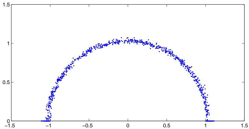
Figure 3: Here we reused the sample used for figure 2. The graphic is a plot of the 1000 i.i.d. realizations of the sub-dominant eigenvalue \lambda_2(\sqrt{n} \mathbf{M}) . Since we deal with real matrices, the spectrum is symmetric with respect to the real axis, and we plotted (\text{RealPart}(\lambda_2), |\text{ImaginaryPart}(\lambda_2)|) in the complex plane.
