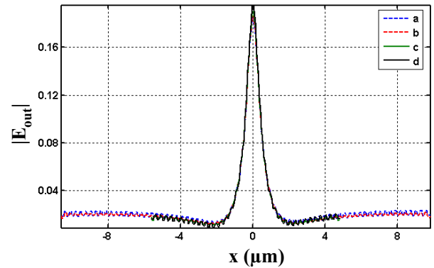
FIG. 11 Influence of the computational window and of the absorbing boundaries on |E_x| obtained with the MM4 in the horizontal plane located at 400nm below the silver interface. The computational window is 20.5 \mu\text{m} for (a) and (b), 10.5 \mu\text{m} for (c) and (d). The three angles for zero reflection are [0^\circ, 0^\circ, 0^\circ] for (b) and (c), and [0^\circ, 80^\circ and 85^\circ] for (a) and (d).
