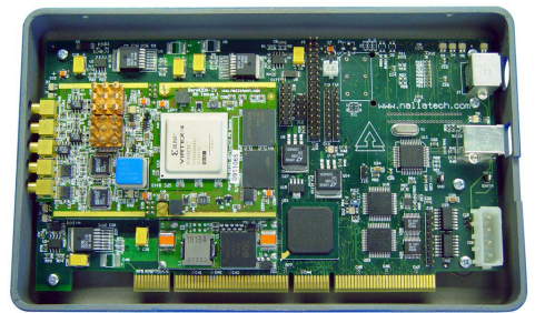
Figure 3. XtremeDSP Development board for Virtex-4.
