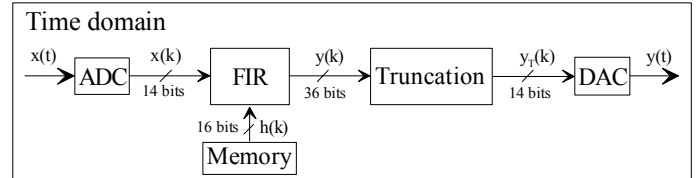
Figure 7. Time domain block diagram for a one-way SISO channel.
