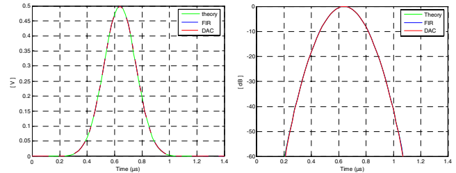
Figure 8. Time domain output signal in linear and log scale.
