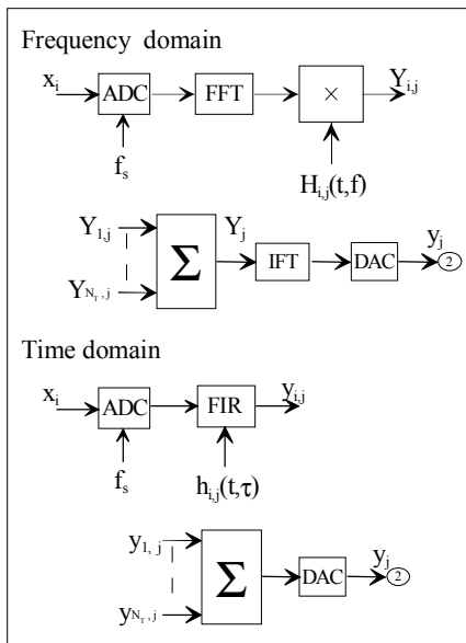
Figure 2. Digital block.
