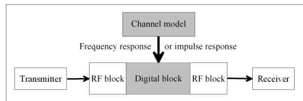
Figure 1. Block diagram of a one-way SISO channel.
