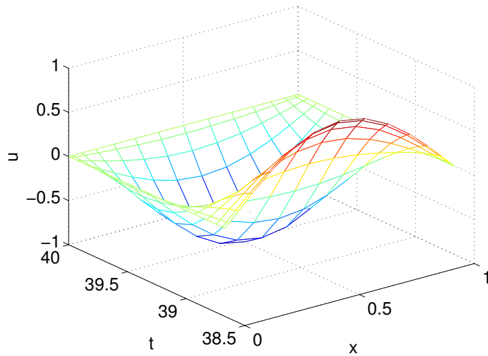
Figure 2: The numerical solution computed at the last time interval, i.e., for 38.6666 \leq t \leq 40 ( T = 4/3 ). The polynomial degree in both the spatial and temporal direction is N = 15 . The error in the discrete L^2 norm is 3.6 \cdot 10^{-12} .
