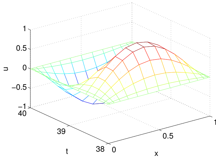
Figure 1: The numerical solution computed at the last time interval, i.e., for 38 \leq t \leq 40 ( \Delta T = 2 ). The polynomial degree in both the spatial and temporal direction is N = 15 . The error in the discrete L^2 norm is 2.1 \cdot 10^{-9} .
