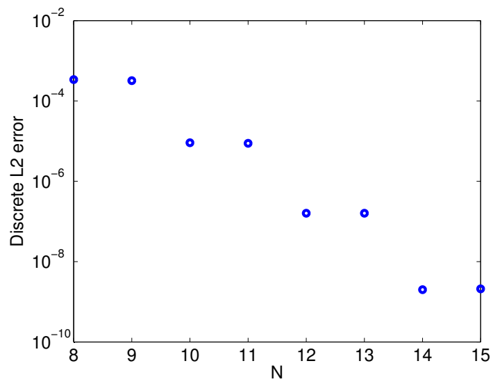
Figure 3: Convergence results for the convection-diffusion problem. The size of each spectral element in the time direction is T = 2 .
