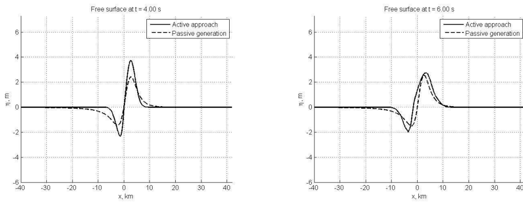
Figure 5: Same as Figure 4 for times t = 4 s and t = 6 s.
