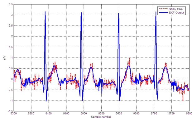
Figure 2. EKF output for ECG signals with erased
