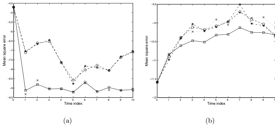
Fig. 4. Plot of MSE performances (on log-scale) of the bootstrap particle filter (*), the SSAPF based on optimal weights (□), the SSAPF based on the generic weights t_k^{\text{P\&S}} (○), and the fully adapted SSAPF (×) for the ARCH model in Section 5.1. The MSE values are computed using 10,000 particles and 400 runs of each algorithm.
