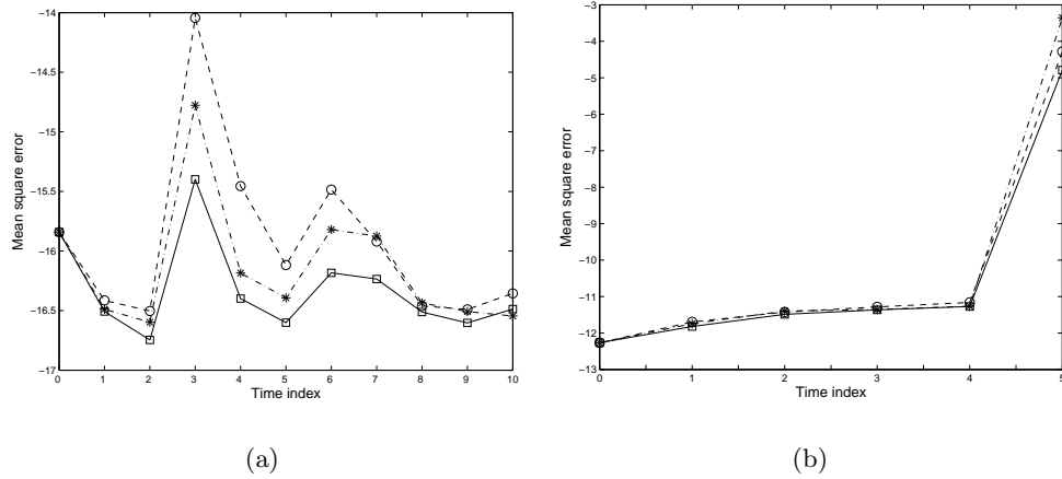
Fig. 1. Plot of MSE performances (on log-scale) of the bootstrap particle filter (*), the SSAPF based on optimal weights (□), and the SSAPF based on the generic weights t_k^{P\&S} of Pitt and Shephard (1999a) (○). The MSE values are founded on 100,000 particles and 400 runs of each algorithm.
