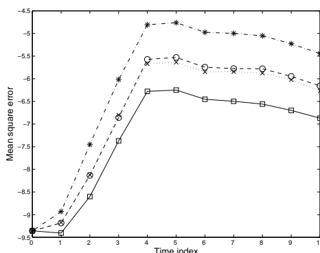
Fig. 5. Plot of MSE performances (on log-scale) of the bootstrap particle filter (*), the SSAPF based on optimal weights (□), the SSAPF based on the generic weights t_k^{\text{P\&S}} (○), and the fully adapted SSAPF (×) for the SV model in Section 5.2. The MSE values are computed using 5,000 particles and 400 runs of each algorithm.
