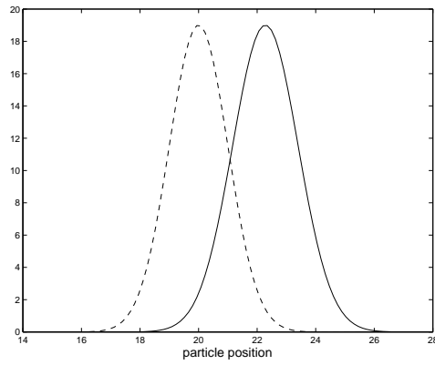
Fig. 2. Plot of the first-stage importance weight functions t_4^* (unbroken line) and t_4^{P\&S} (dashed line) in the presence of an outlier.
