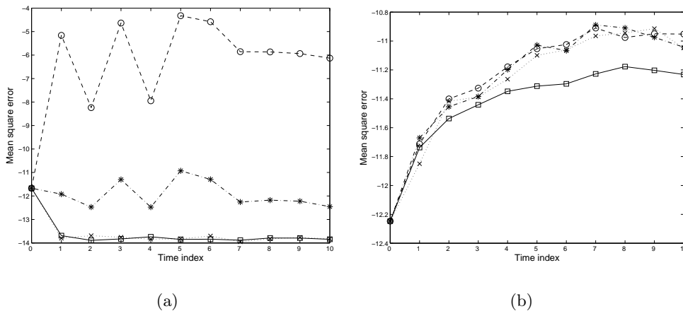
Fig. 3. Plot of MSE performances (on log-scale) of the bootstrap particle filter (*), the SSAPF based on optimal weights (□), the SSAPF based on the generic weights t_k^{P\&S} (○), and the fully adapted SSAPF (×) for the Linear/Gaussian model in Section 5.1. The MSE values are computed using 10,000 particles and 400 runs of each algorithm.
