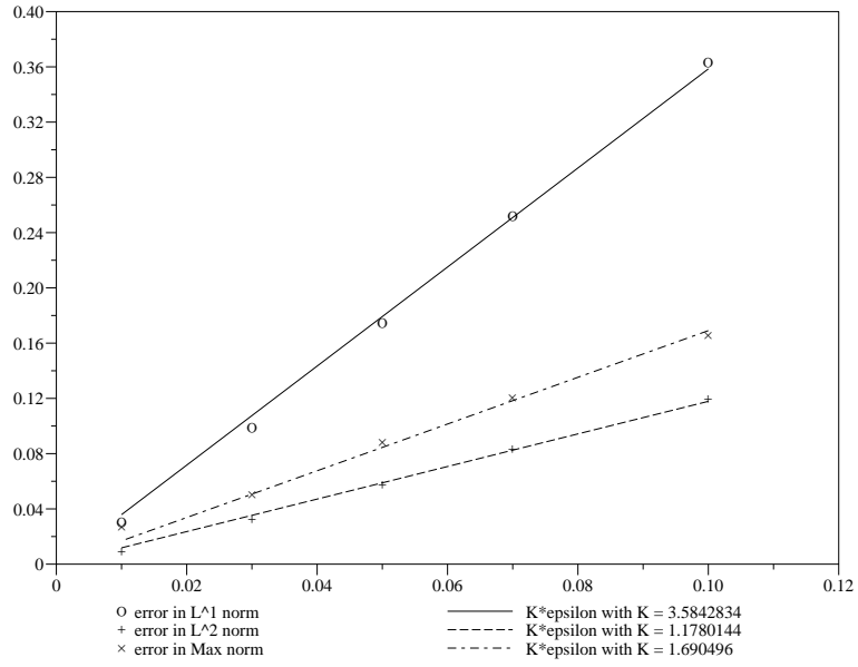
Figure 4: Error u^\epsilon(x, t) - U_h(x, \frac{t}{\epsilon}, t) in L^1 , L^2 and L^\infty norms.
