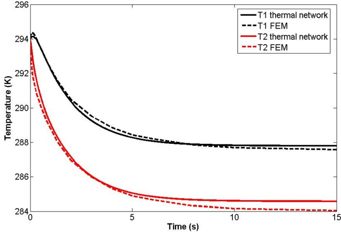
Fig. 8. T_1 et T_2 for the geometry I in water
