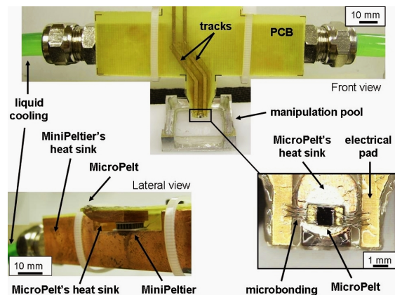
Fig. 3. Experimental freeze gripper.
