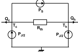
Fig. 5. Thermal network for a Peltier element [8].
