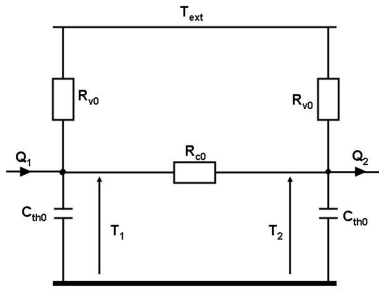
Fig. 7. Thermal network for the heat sinks and the end-effector.
