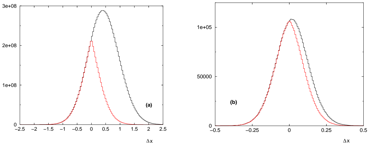
FIG. 3: (Color online) Monte-Carlo procedure to measure the negative tail on x \in [-11, -1] in d = 1 : histograms of the proposed and accepted Monte-Carlo changes \Delta x in the disorder (a) for L = 25 where the acceptance rate is \tau_{acc} \sim 0.425 (b) for L = 1600 where the acceptance rate is \tau_{acc} \sim 0.86 .
