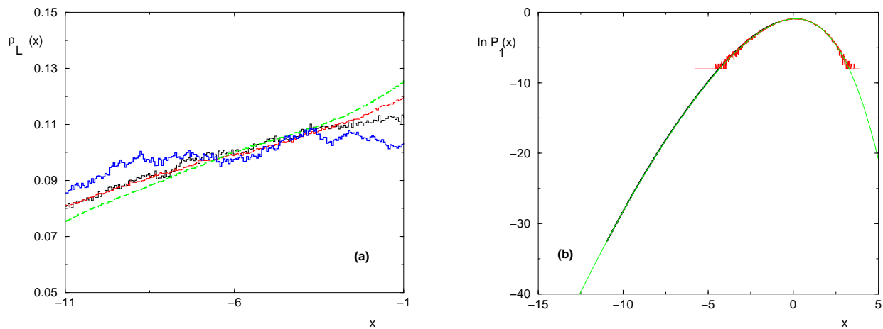
FIG. 5: (Color online) Monte-Carlo procedure to measure the negative tail on x \in [-11, -1] in d = 1 : (a) relative histogram \rho_L(x) = P_L(x)/P_{TW}^{GOE}(x) with respect to the exact guiding function : convergence towards the flat histogram as L grows : L = 200 (dashed line), 400, 800, 1600 (thick line). (b) logarithmic plot of the negative tail of the probability distribution P_1(x) , as compared to simple sampling result for L = 1600 . The exact Tracy-Widom distribution is also shown (thin line) to demonstrate the validity of the Monte-Carlo procedure.
