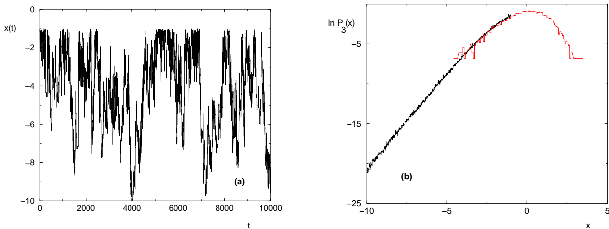
FIG. 7: (Color online) Monte-Carlo procedure to measure the negative tail on x \in [-10, -1] in d = 3 for L = 72 : (a) process x(t) during the first 1 \leq t \leq 10000 Monte-Carlo iterations (b) logarithmic plot of the negative tail of the probability distribution P_3(x) , as compared to simple sampling result.
