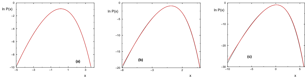
FIG. 2: (Color online) Fits of the GOE Tracy-Widom distribution \ln P_{TW}^{GOE}(x) by generalized Gumbel distributions \ln g_m(x) (Eq. 22) on various intervals : (a) fit on [-5, 3.7] corresponding to \ln P > -10 with m = 12.93 ; (b) fit on [-8, 5] corresponding to \ln P > -20 with m = 14.71 (c) fit on [-10, 6] corresponding to \ln P > -30 with m = 15.92 ;
