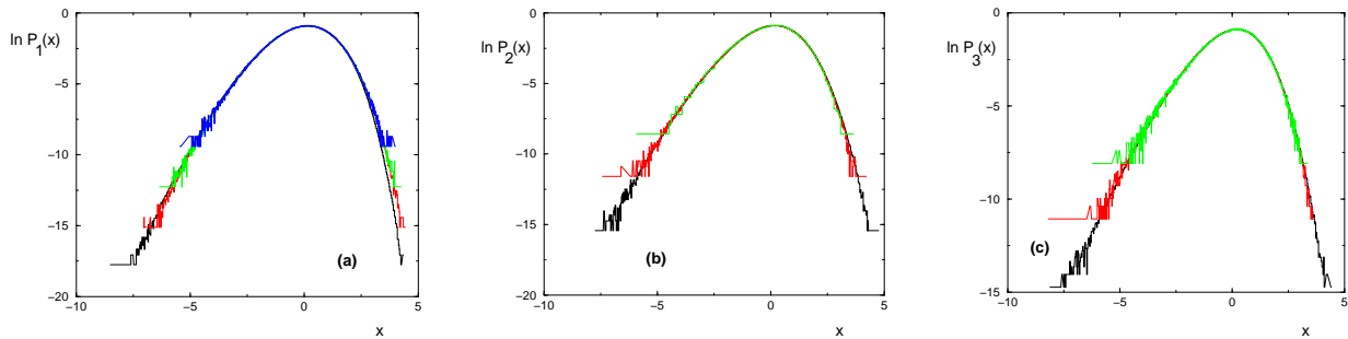
FIG. 1: (Color online) Logarithmic plot of the rescaled probability distribution P_d(x) (Eq. (1)) as measured via simple sampling for (a) L = 12, 50, 200, 800 in d = 1 ; (b) L = 10, 40, 160 in d = 2 ; (c) L = 6, 18, 36 in d = 3
