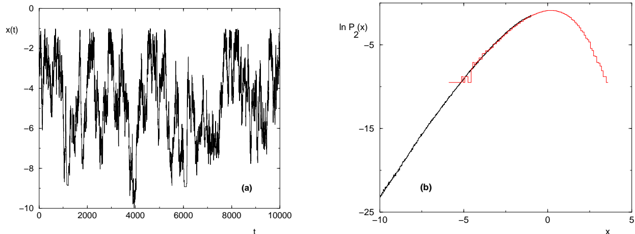
FIG. 6: (Color online) Monte-Carlo procedure to measure the negative tail on x \in [-10, -1] in d = 2 for L = 120 : (a) process x(t) during the first 1 \leq t \leq 10000 Monte-Carlo iterations (b) logarithmic plot of the negative tail of the probability distribution P_2(x) , as compared to simple sampling result.
