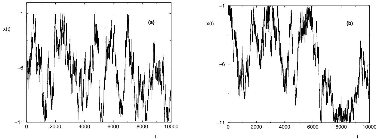
FIG. 4: (Color online) Monte-Carlo procedure to measure the negative tail on x \in [-11, -1] in d = 1 : process x(t) during the first 1 \leq t \leq 10000 Monte-Carlo iterations (a) for L = 50 (b) for L = 200
