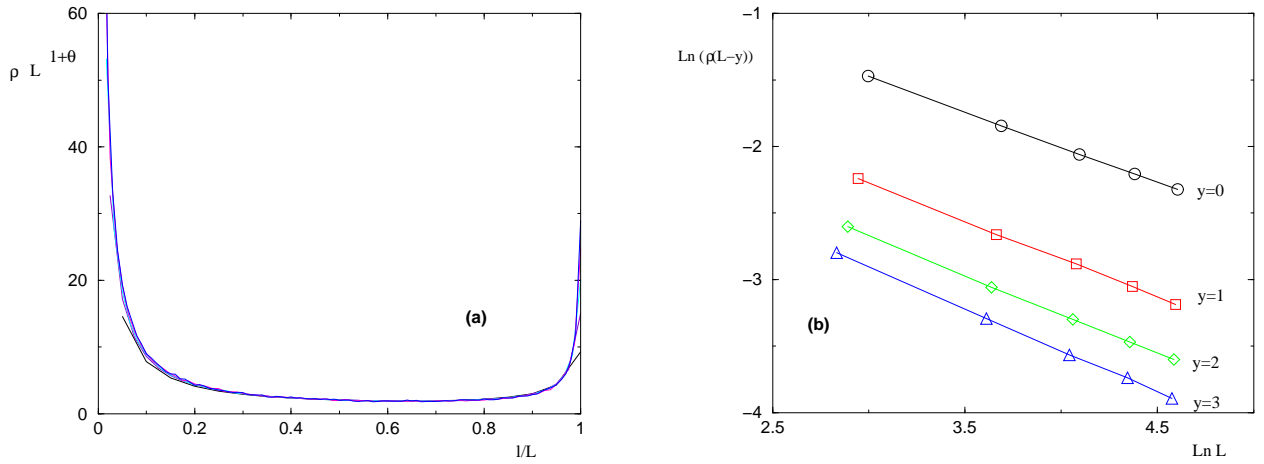
FIG. 7: d = 2 : (a) Rescaled distribution R^{\text{boundary}}(x = l/L) (see equation (32)), that is singular for x \rightarrow 0 and x \rightarrow 1 . (b) Log-log plot of the density \rho_L^{\text{boundary}}(E = 0, l = L - y) of very large boundary excitations l = L - y with finite y = 0, 1, 2, 3 .
