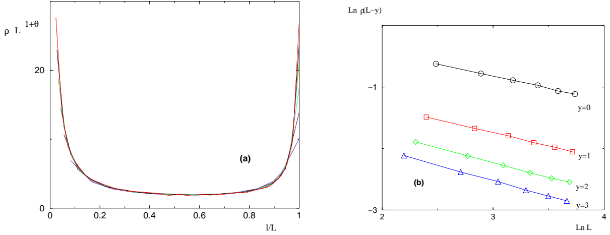
FIG. 9: d = 3 : (a) Rescaled distribution R^{boundary}(x = l/L) (see equation (37)), that is singular for x \rightarrow 0 and x \rightarrow 1 . (b) Log-log plot of the density \rho_L^{boundary}(E = 0, l = L - y) of very large boundary excitations l = L - y with finite y = 0, 1, 2, 3 .
