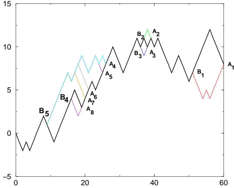
FIG. 10: Notion of independent bulk excitations (in d = 1 ) : for each sample, we generate the ground state (bold line) and consider all points A_i of the ground state, with partial energy E_0(A_i) . When the energy E_1(A_i) of the second best path ending at A_i satisfies E_1(A_i) - E_0(A_i) < T , we construct these bulk excitations (light lines) that join again the ground state at some branch point B_j . These bulk excitations tend to cluster into families. In our counting procedure of independent excitations, two excitations are independent if they have no bond in common. For instance on the Figure, end-points A_4 , A_5 , A_6 and A_7 count for a single excitation associated to the branch point B_5 . The other independent excitations are (A_1, B_1) , (A_2, B_2) , (A_3, B_3) and (A_8, B_4) .
