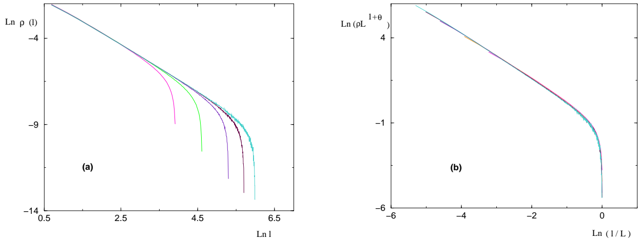
FIG. 11: (a) Log-log plot of the density \rho_L^{bulk}(E = 0, l) of boundary excitations of length l in d = 1 for L = 50, 100, 200, 300, 400 . (b) Same data after the rescaling of equation (43) with exponent \theta_1 = 1/3 .
