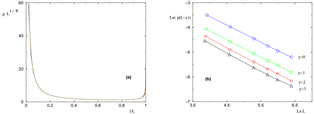
FIG. 5: d = 1 : (a) Rescaled distribution R^{boundary}(x = l/L) (see equation (27)), that is singular for x \rightarrow 0 and x \rightarrow 1 . (b) Log-log plot of the density \rho_L^{boundary}(E = 0, l = L - y) of very large boundary excitations l = L - y with finite y = 0, 1, 2, 3 .
