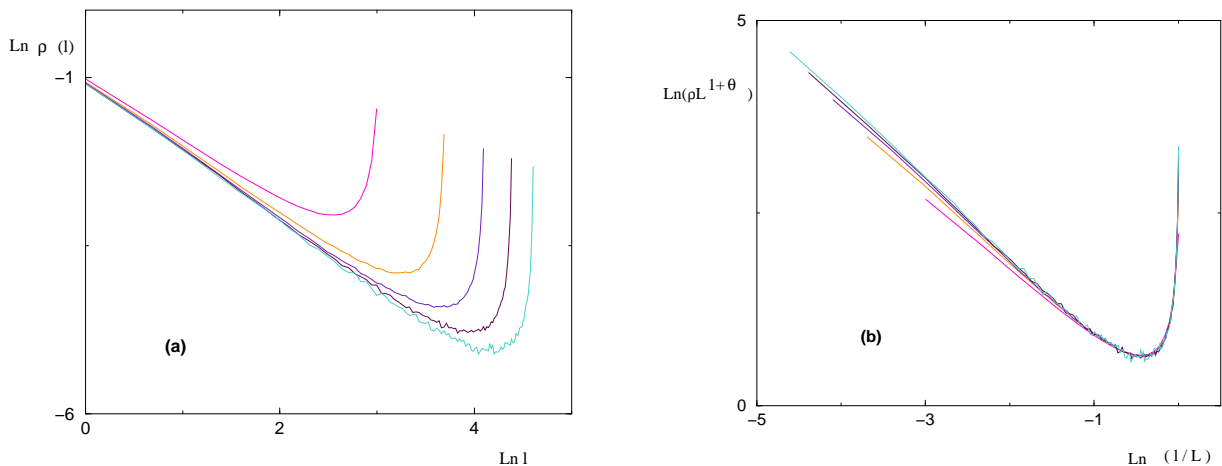
FIG. 6: (a) Log-log plot of the density \rho_L^{boundary}(E=0, l) of boundary excitations of length l in d = 2 for L = 20, 40, 60, 80, 100 . (b) Same data after the rescaling of equation (32) with \theta_2 \sim 0.24 .
