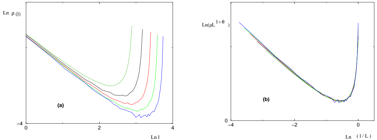
FIG. 8: (a) Log-log plot of the density \rho_L^{\text{boundary}}(E = 0, l) of boundary excitations of length l in d = 3 for L = 18, 24, 30, 36, 42 (b) Same data after the rescaling of equation (37) with \theta_3 \sim 0.18 .
