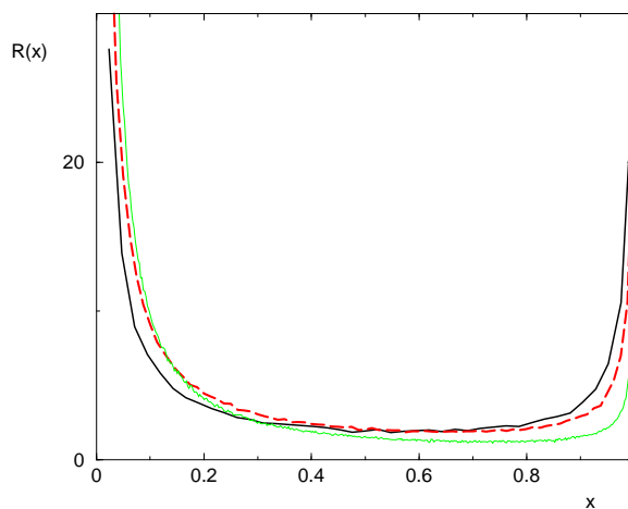
FIG. 14: Comparison of the scaling function R^{boundary}(x) for d = 1 (thin line), d = 2 (dashed line) and d = 3 (thick line).
