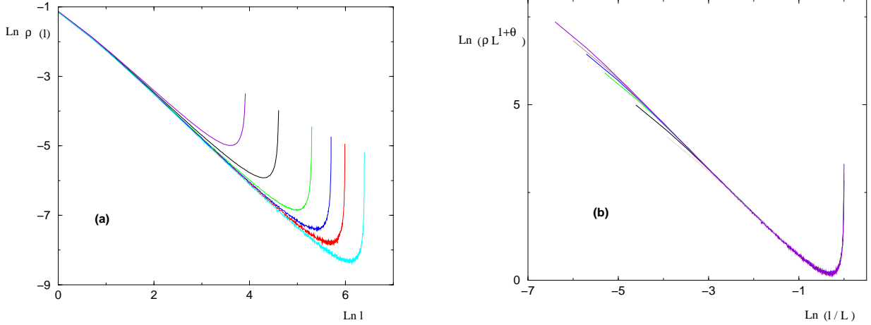
FIG. 4: (a) Log-log plot of the density \rho_L^{boundary}(E = 0, l) of boundary excitations of length l in d = 1 for L = 50, 100, 200, 300, 400, 600 . (b) Same data after the rescaling of equation (27) with \theta_1 = 1/3 .
