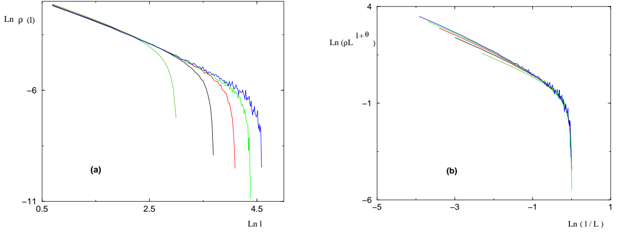
FIG. 12: (a) Log-log plot of the density \rho_L^{bulk}(E=0, l) of boundary excitations of length l in d=2 for L=20, 40, 60, 80, 100 . (b) Same data after the rescaling of equation (43) with exponent \theta_2=0.24 .
