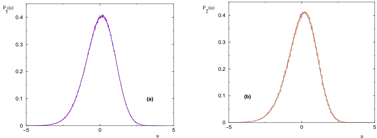
FIG. 1: (a) Rescaled distribution F_1(u) of the d = 1 ground state energy (see equation (17)), for L = 50, 100, 200, 300, 400, 600 . (b) Rescaled distribution F_2(u) of the d = 2 ground state energy (see equation (17)), for L = 10, 20, 40, 80, 120 .
