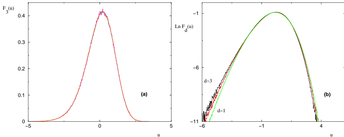
FIG. 2: (a) Rescaled distribution F_3(u) of the d = 3 ground state energy (see equation (17)), for L = 6, 12, 18, 24, 36 . (b) Comparison of \text{Ln } F_d(u) for d = 1, 2, 3 (see equation (17)).
