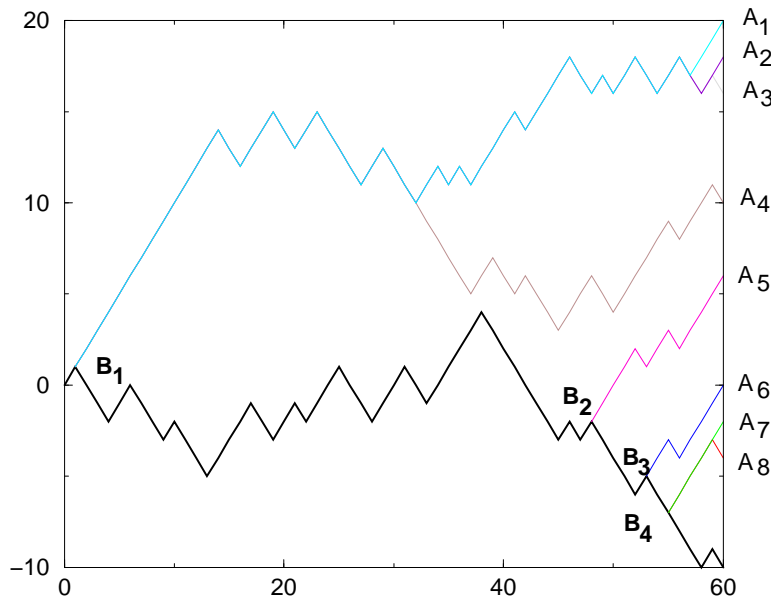
FIG. 3: Notion of independent boundary excitations (in d = 1 ) : for each sample, we generate the ground state (bold line) of energy E_0 , and consider all end-points A_i where the energy E(A_i) of the best path ending at A_i satisfies E(A_i) - E_0 < T (light lines). These best paths tend to cluster into families. In our counting procedure of independent excitations, two excitations are independent if they have no bond in common. For instance on the Figure, end-points A_1, A_2, A_3 and A_4 count for a single excitation associated to the branch point B_1 . Similarly A_7 and A_8 count for a single excitation associated to the branch point B_4 .
