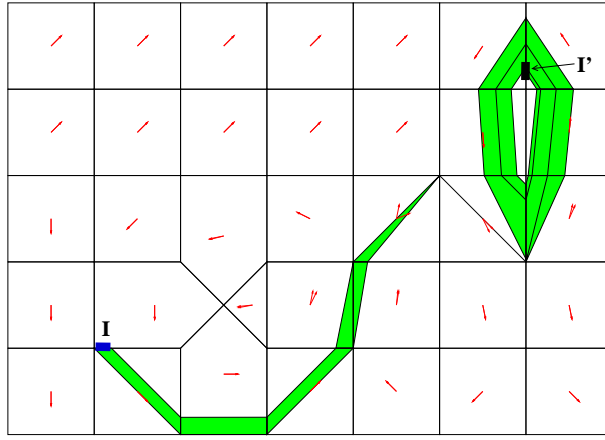
Fig. 2. Reachability analysis.
