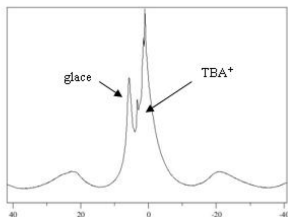
Figure 12 : Spectre RMN MAS ( \nu_{rot}=6kHz ) du semi clathrate D_2O-TBABr .
