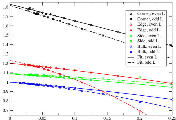
FIG. 6: Normalized probabilities for an end point being a corner site ( p_C ), an edge site ( p_E ), a side site ( p_S ), or a bulk site ( p_B ), as functions of 1/L .
