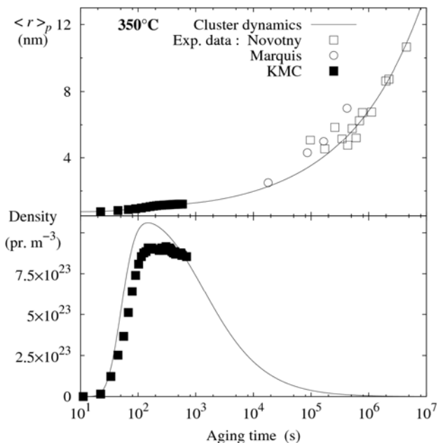
Figure 2: Mean radius and number density of precipitates as a function of the aging time for the Al Sc 0.18 at%Sc solid solution aged at 350°C as given by cluster dynamics and by Kinetic Monte Carlo. Experimental results are also reported [7-8].
