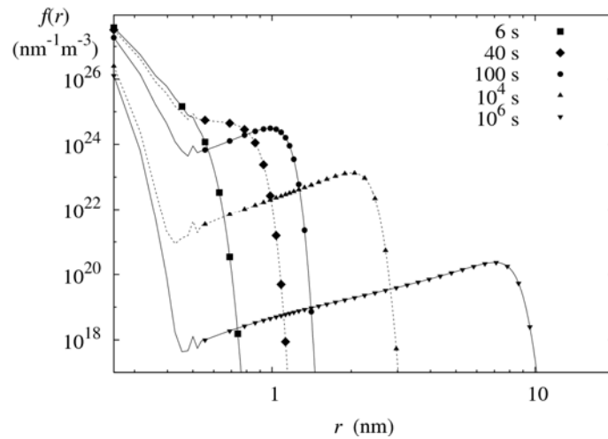
Figure 1: Size histogram evolution of Al 3 Sc precipitates in the AlSc 0.18at% solid solution thermally treated at 350°C.
