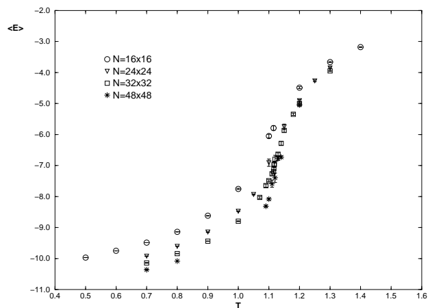
FIG. 1. Averaged energy versus temperature, for N = 16 \times 16 , 24 \times 24 , 32 \times 32 and 48 \times 48
