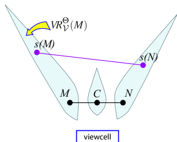
Figure 11: When M and N are moved within their validity region (to s(M) and s(N) respectively) not all points on [MN] can be simplified on [s(M),s(N)] . E.g. C 's validity region does not intersect [s(M),s(N)]
