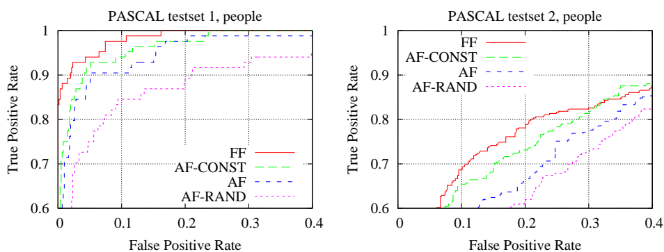
Figure 19: ROC curves of our method on the PASCAL challenge. The method is trained and tested with four combinations of the foreground features with different types of background. The same type of background is used for training and testing.
