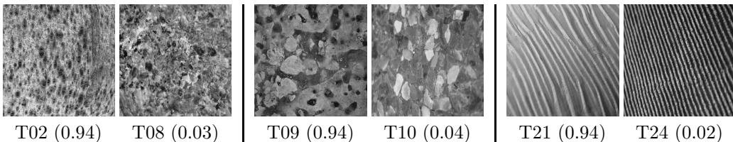
Figure 13: Example images of the most difficult texture classes of UIUC database and their confused classes. The left example of each pair shows the difficult texture class and its classification accuracy. The right example shows the most confused class and the confusion rate for the class on the left.
