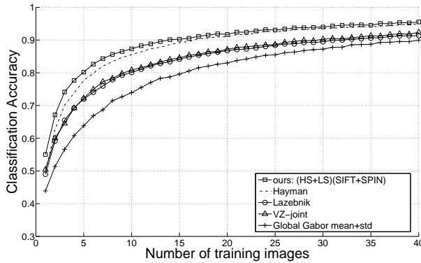
Figure 14: Comparison of different methods on the whole KTH-TIPS texture database
