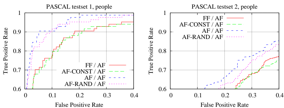
Figure 20: ROC curves of our method on the PASCAL challenge. The method is trained with four combinations of the foreground features with different types of background, and tested on the original test set of the PASCAL challenge.
