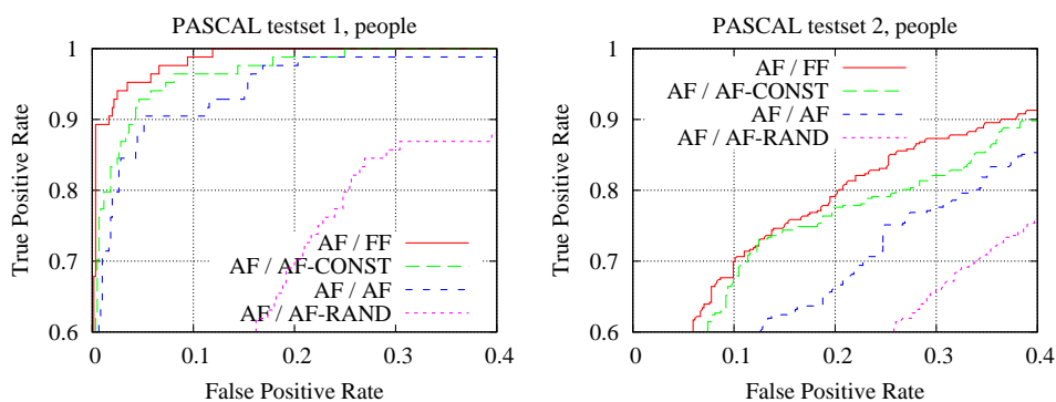
Figure 21: ROC curves of our method on PASCAL challenge. The method is trained on the original training set of PASCAL challenge, and tested on four combinations of the foreground features with different types of background.
