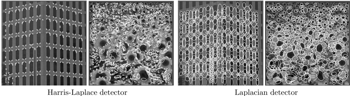
Figure 1: Illustration of affine Harris and Laplacian regions on two natural images.
