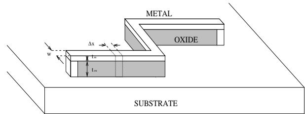
Fig. 1. Interconnect line
