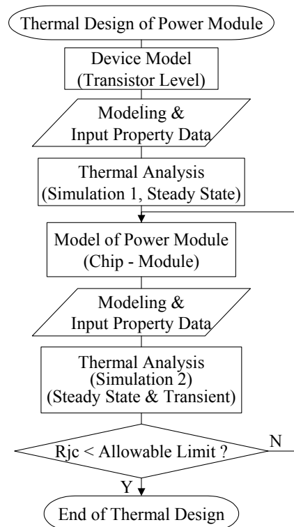
Figure 2 Flow chart illustrating the thermal design of power semiconductor modules on PCB
