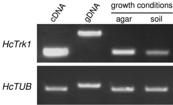
FIGURE 8. HcTrk1 transcripts are present in external hyphae of H. cylindrosporum grown in symbiotic conditions. The symbiotic plant partner of H. cylindrosporum is P. pinaster . The symbionts were grown either on thin layer of forest soil or agar plates. External hyphae were collected for RT-PCR analyses of HcTrk1 transcripts. Reverse transcription was performed using 0.5 \mu g of total RNA. PCR amplifications were performed with either HcTrk1 primers (top panel) or HcTUB primers (bottom panel; control). The number of cycles was 40 for both HcTrk1 and HcTUB , respectively. For both genes the size of the amplified fragments was checked by comparison with DNA fragments obtained in parallel experiments by PCR on the corresponding cDNA or on genomic DNA (first two lanes).
