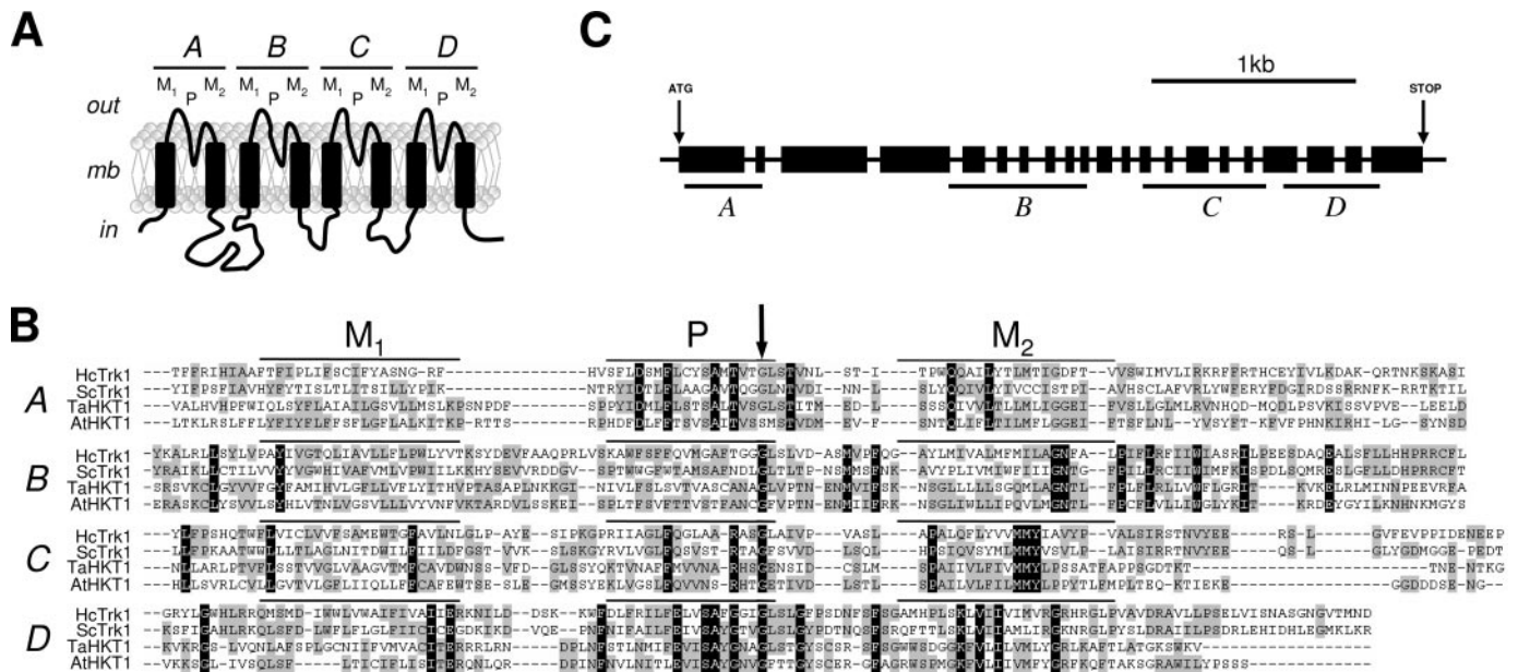
FIGURE 1. Identification of HcTrk1, a Trk transporter in the ectomycorrhizal basidiomycete H. cylindrosporum . A , schematic structural model of Trk transporters. Trk transporters display four tandemly repeated MPM domains (named A–D), each comprising two transmembrane ( mb ) segments ( M 1 and M 2 ) surrounding a pore region ( P ). B , sequence alignments in the regions corresponding to the four MPM motifs of H. cylindrosporum HcTrk1 and of Trk transporters from other fungal or plant species: S. cerevisiae ScTrk1, T. aestivum TaHKT1, and A. thaliana AtHKT1. Identical amino acids are on a black (conserved in all four proteins) or gray background. The arrow indicates a highly conserved residue shown to be essential for transport selectivity (60). C , gene structure of HcTrk1. Exons are designated by black boxes. The mean intron size is 60 bp. kb , kilobase(s).
