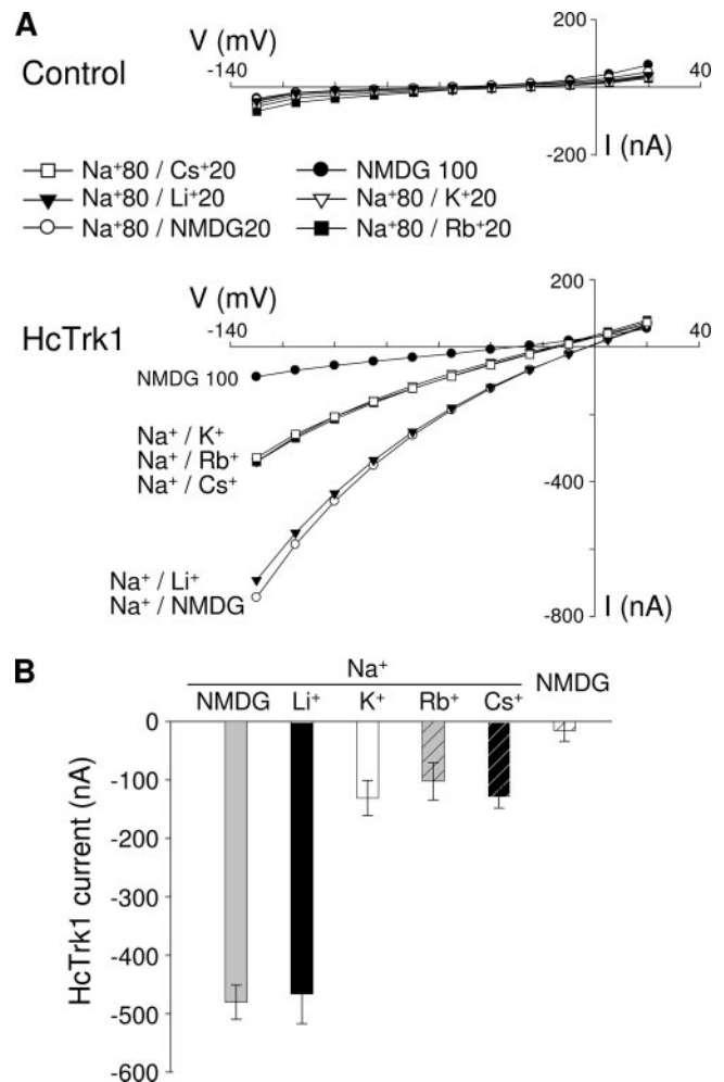
FIGURE 5. Inhibition by K + , Rb + , and Cs + of HcTrk1 currents in presence of Na + . The bath solution contained a total monovalent cations concentration of 100 mM: 80 mM Na + and 20 mM X (X is either K + , Rb + , Cs + , Li + , or NMDG) or 100 mM NMDG in the standard background medium. A , representative I-V curves recorded in a control oocyte injected with water (upper panel) or in a HcTrk1-expressing oocyte (lower panel). B , mean HcTrk1 current at -115 mV. Bath solutions as in A . Each bar represents the mean HcTrk1 current (± S.D.; n = 4). HcTrk1 current, total current in HcTrk1-expressing oocyte minus mean control current obtained from three water-injected oocytes in parallel experiments.
