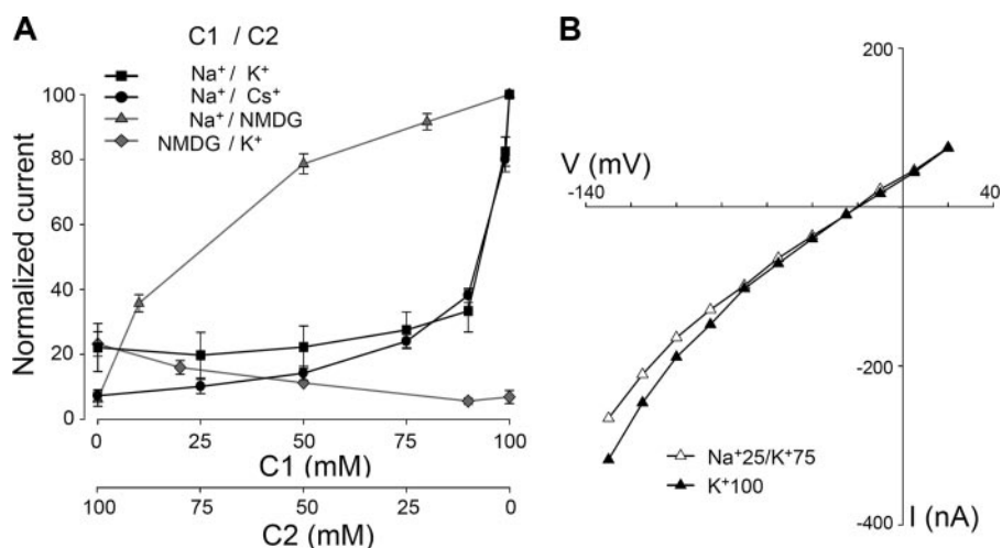
FIGURE 6. Interaction between Na + and K + in HcTrk1 revealed by anomalous mole fraction effect. A , the bath solution contained in the standard background medium a mix of two monovalent cations, C1 and C2, for a total concentration of 100 mM: Na + and NMDG (gray triangles; data from the same experiments as in Fig. 3), Na + and K + (black squares), Na + and Cs + (black circles), and NMDG and K + (gray diamonds; data from the same experiments as in Fig. 3), as C1 and C2 respectively. For each oocyte in each bath solution, the HcTrk1 current was obtained by subtracting from the total current the mean control current recorded in three water-injected oocytes in parallel experiments. Normalized HcTrk1 current is HcTrk1 current at -115 mV in a given bath expressed as a percentage of the HcTrk1 current recorded at the same potential in 100 mM Na + . Data of the means ( \pm S.D.) obtained from 4–8 HcTrk1-expressing oocytes. B , HcTrk1 current magnitude is lower in 25 mM Na + /75 mM K + than in 100 mM K + . Current/voltage curves in 100 mM K + or 25 mM Na + /75 mM K + were obtained in a representative HcTrk1-expressing oocyte. Independent experiments performed on 12 oocytes displaying different levels of HcTrk1 currents systematically revealed that the increase in Na + mole fraction from 0 (100 mM K + solution) to 0.25 (25 mM Na + /75 mM K + solution) resulted in decreased current magnitudes at every membrane potential. Wilcoxon signed-rank test indicates that this decrease in current magnitude upon the increase in Na + mole fraction was statistically significant ( p \ll 0.01 ).
