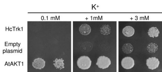
FIGURE 2. HcTrk1 complements S. cerevisiae mutant cells defective for K + uptake. Cells from the yeast mutant strain WΔ6 ( trk1 -Δ::LEU2 trk2 -Δ::HIS3) defective for K + uptake were transformed with either HcTrk1 cDNA cloned in the yeast expression plasmid pDR196 or the empty plasmid or with the A. thaliana K + channel AKT1 cDNA as a positive control. Drop tests were performed on arginine phosphate medium containing about 0.1 mM K + (nominal concentration) or on AP medium supplemented with 1 or 3 mM KCl. The plates were incubated for 3 days at 30 °C.
