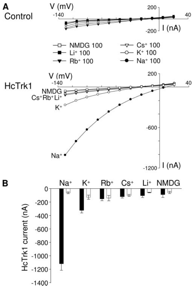
FIGURE 4. HcTrk1 selectivity for alkali cations. The bath solution contained 100 mM concentrations of either Li + , Na + , K + , Rb + , Cs + , or NMDG in the standard background medium. A , representative current-voltage (I-V) curves recorded in a control oocyte injected with water (upper panel) or in a HcTrk1-expressing oocyte (lower panel). B , mean steady state current recorded at -130 mV in HcTrk1-expressing oocytes (black bars) compared with water-injected (control) oocytes (white bars). Bath solutions are as in A . Data are mean values ± S.D. for four oocytes.
