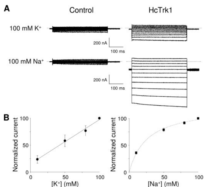
FIGURE 3. HcTrk1 expressed in Xenopus oocytes mediates K + and Na + transport. A, examples of current traces recorded in control oocytes (injected with water, left panels) or in HcTrk1 -expressing oocytes (right panels) recorded in 100 mM KCl (upper panels) or in 100 mM NaCl (lower panels). The voltage step ranged between +20 mV and –130 mV in –15-mV steps from a holding potential of –40 mV. B, effect of K + or Na + concentration on HcTrk1 current. For each oocyte in each bath solution, the HcTrk1 current was defined as the total current in HcTrk1 -expressing oocyte minus the control current (mean current obtained for three control oocytes from the same batch in the same bath). The bath solution contained 1 mM CaCl 2 , 1.5 mM MgCl 2 , 10 mM MES, 5 mM Tris, pH 6.5, as standard background medium, and 10, 50, 80, or 100 mM KCl (left panel) or NaCl (right panel). The ionic strength of the solutions was kept constant by adding N -methyl-D-glucamine to compensate for the change in K + or Na + concentration (no added NMDG in 100 mM K + and in 100 mM Na + ). Normalized HcTrk1 current was HcTrk1 current at –115 mV in the presence of a given concentration of K + (Na + ) expressed as percent of the HcTrk1 current recorded at the same potential in 100 mM K + (Na + ). Data are the means (± S.D.) obtained from 8–12 HcTrk1 -expressing oocytes.
