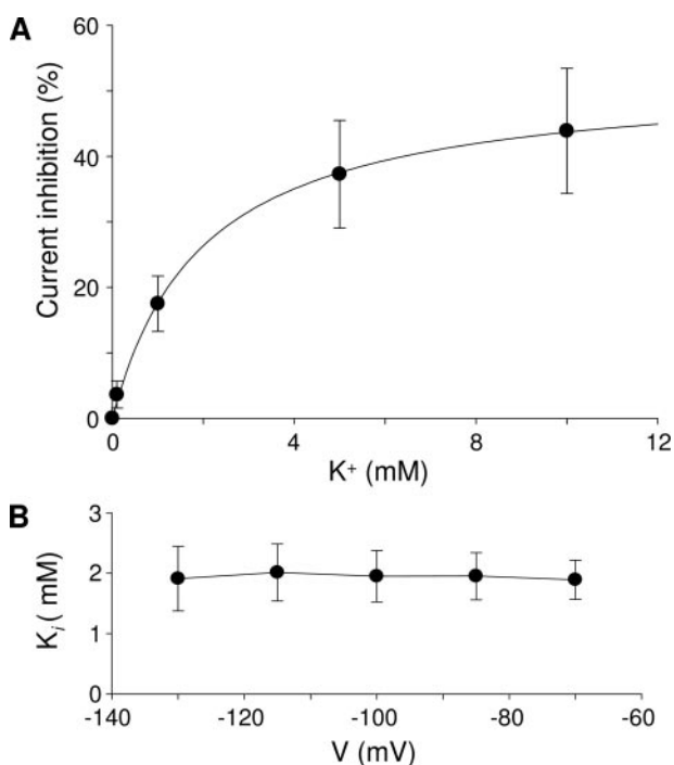
FIGURE 7. K + inhibition of HcTrk1 currents. The bath solution contained 80 mM Na + and either 0, 0.1, 1, 5, or 10 mM K + in the standard background medium. A , HcTrk1 current inhibition was expressed as a percentage of HcTrk1 current recorded at -115 mV in 80 mM Na + . These percentages were fitted to a Michaelis function to derive a K i value. Mean values \pm S.D. for four oocytes. The ionic strength of the solutions was kept constant to 100 mM by adding N -methyl-D-glucamine to compensate for the change in K + . B , K + inhibition of HcTrk1 current in presence of Na + is not sensitive to voltage. Michaelis hyperbolic functions were used to derive inhibition constants K i as described in A at -70, -85, -100, -115, and -130 mV. Data are the means \pm S.D. for four oocytes.
