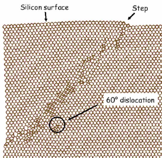
Fig. 2. Cross-section view of a silicon surface with a monoatomic step, submitted to a uniaxial compression of 10% (disoriented by 22.5^\circ with respect to the step line), after relaxation at 0K
