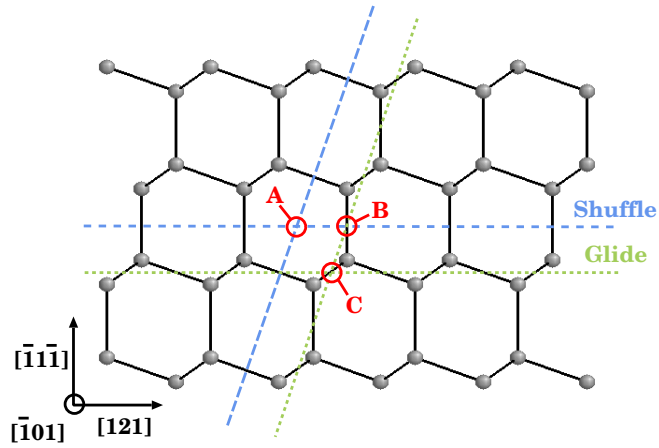
FIG. 1: Ball-and-stick representation of the cubic diamond structure, oriented along axis X = [121] , Y = [\bar{1}\bar{1}\bar{1}] and Z = [\bar{1}01] . Shuffle and glide sets of planes are shown, as well as the three possible stable locations A, B, and C for a screw dislocation in silicon [14].
