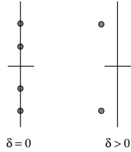
FIG. 2: Schematic of the effect of dissipation on the eigenvalues associated with (2).
