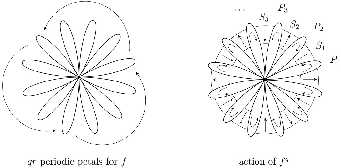
Figure 1: Local topological dynamics of f : z \mapsto e^{2i\pi\frac{p}{q}}z(1+z^{qr}) ; here q = 3 , p = 1 , r = 2 , so that there is two orbits of attracting petals and two orbits of repulsive petals
