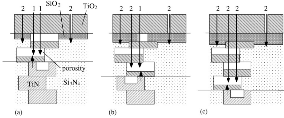
Fig. 7. Evolution of oxidation mechanisms during the second oxidation mode.
