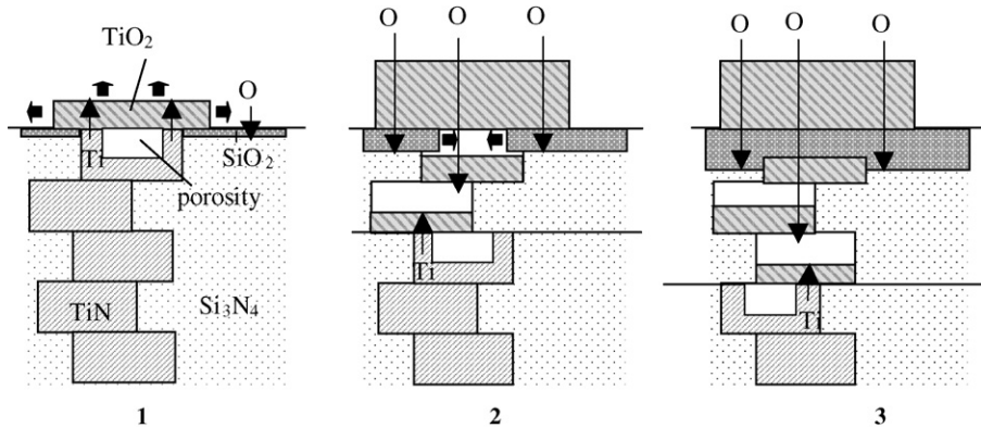
Fig. 6. The three steps of the oxidation model for temperature >1000 °C.
