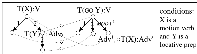
Fig. 5. Translation (6) and the corresponding restructuring rule.
