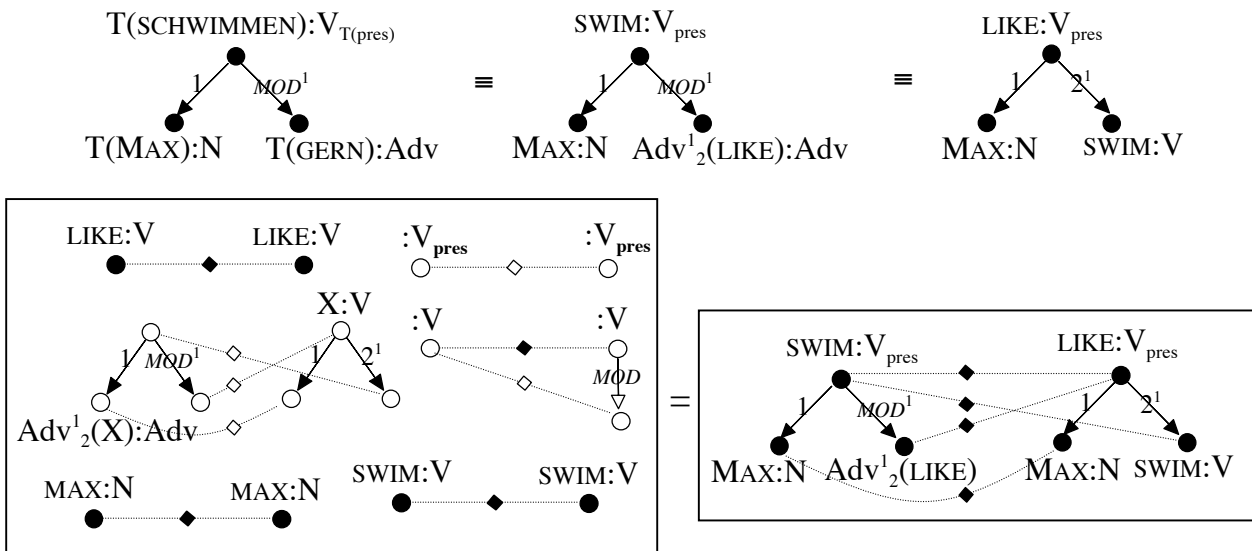
Fig. 4. The translation (4)
