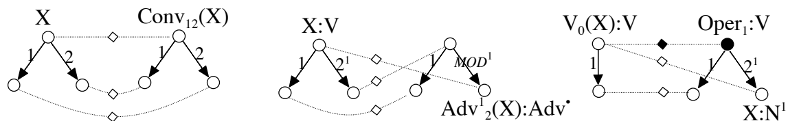
Fig. 2. Restructuring rules associated with \text{Conv}_{12} , \text{Adv}_{12}^1 and \text{Oper}_1
