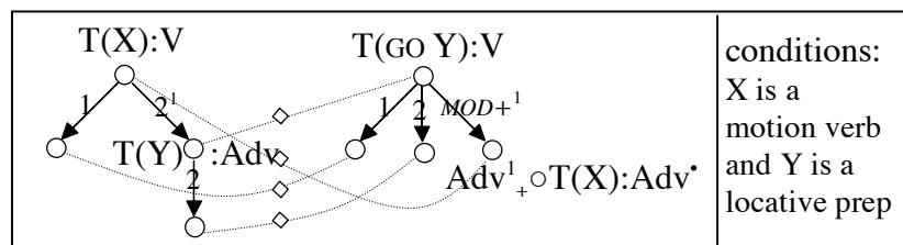
Fig. 5. Translation (6) and the corresponding restructuring rule.
