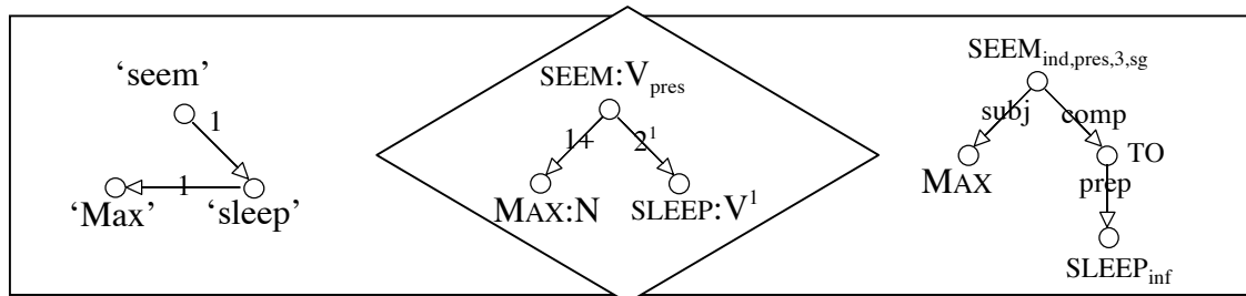
Fig. 1 The SemS, DSyntS et SSyntS of Max seems to sleep
