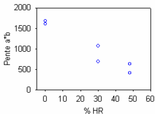
Fig.8: Variation of ' a*b ' with the relative humidity of the gas mixtures. The content of formaldehyde was kept equal to 2 ppb and the flux was 220 \text{ mL}\cdot\text{min}^{-1} .
