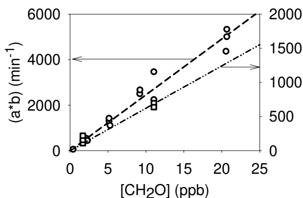
Fig. 7. Calibration curves for the quantitative determination of formaldehyde. Relative humidity: left = 0, right = 45%.
