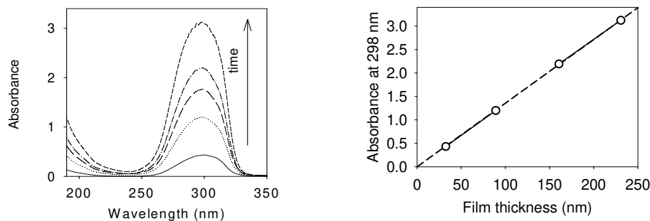
Fig. 2. Variation of the absorbance of the thin film doped with Fluoral-P as a function of the maturation time of the sol, respectively 180, 220, 230, 240 and 245 minutes (left) and thickness of the thin film (right). The absorption coefficient of Fluoral-P at 298 nm is 16800 \pm 900 \text{ mol}^{-1} \cdot \text{L} \cdot \text{cm}^{-1} .
