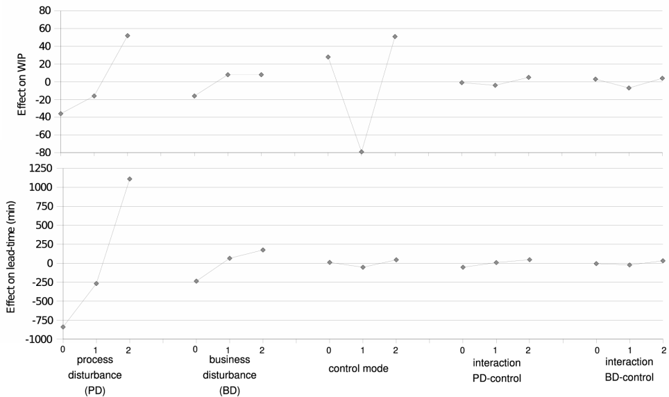
Figure 1: Effects on WIP and lead time
