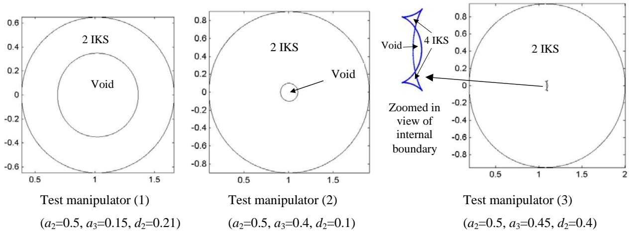
(b) Workspaces of the test manipulators
