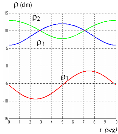
Figure 10: Joint trajectories by using Global Minimization of \kappa(J) .
