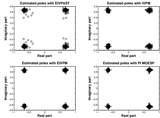
Figure 1. Estimated poles obtained with IVPM, EIVPM, EIVPAST and PI MOESP algorithms for a Monte Carlo simulation of size 100.
