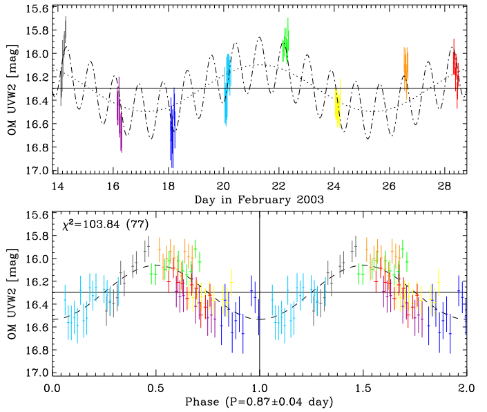
Fig. 5. Weekly and daily UV variability of AA Tau observed with the OM. Top panel: the dotted and dashed-dotted line show the weekly modulation of the UV flux attributed to the eclipse period (8.22 days), and the overall modulation of the UV flux. The horizontal line shows the average flux. Bottom panel: the dashed line shows the daily modulation of the UV folded in phase after subtraction of the weekly modulation. Symbols are the same in both panels. The formula of the overall fit (dashed-dotted line) is given by Eq. 1.
