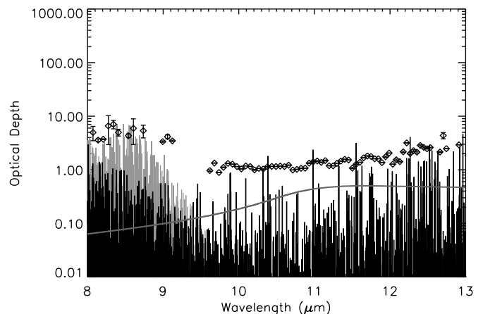
Fig. 4. Optical depths observed with MIDI (black diamonds) and high-resolution opacity profiles of water (black), SiO (grey) and alumina (solid grey line).
