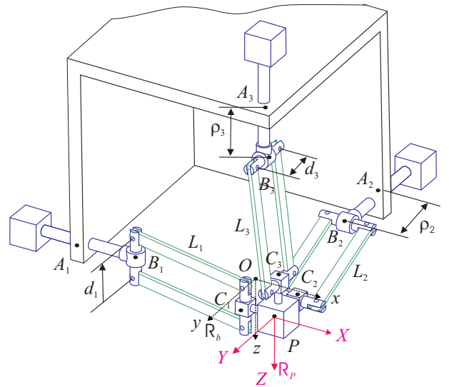
Figure 1. Basic kinematic architecture of the Orthoglide
