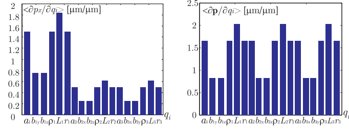
Figure 14. Q_2 configuration, sensitivity of p_x
