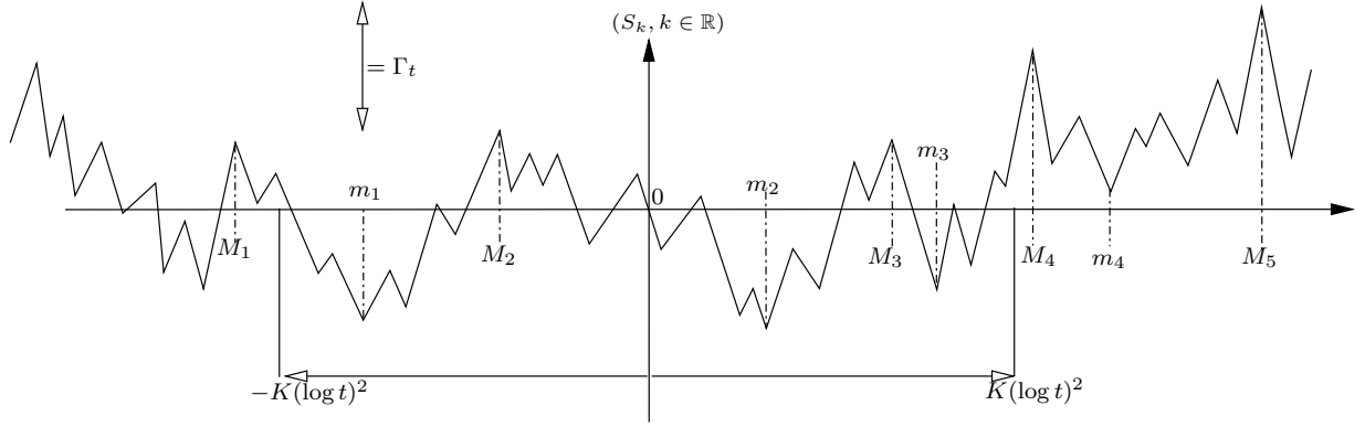
Figure 3: Support of f and the valleys
