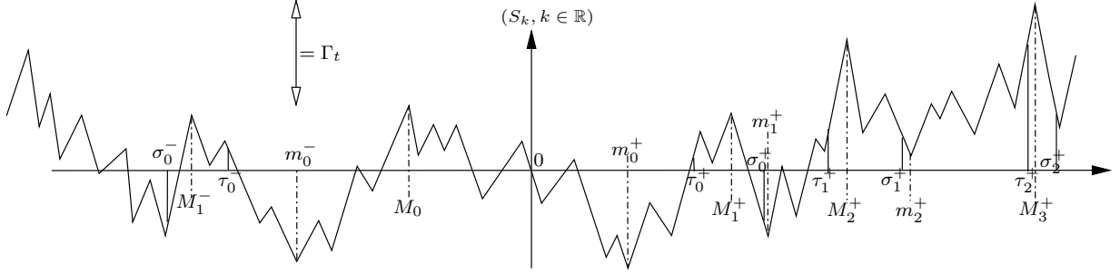
Figure 2: Construction of the valleys 2/2
