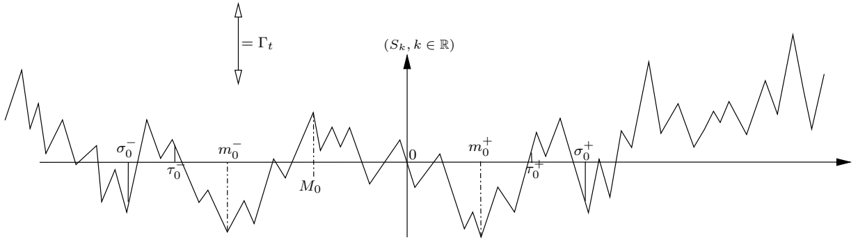
Figure 1: Construction of the valleys 1/2
