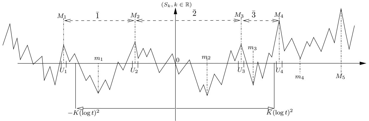
Figure 4: Random cover and sets of indeterminate points with n(f) = 3 .
