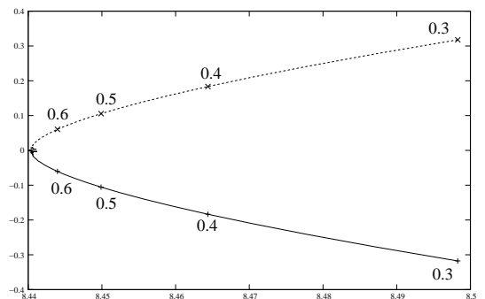
Figure 3: Solutions of the dispersion relation in the \alpha complex plane for different values of h , which is given for some points as a fraction of the wavelength. The waveguides are characterized by h_1 = 0.2 \lambda , \epsilon_1 = 3 , \mu_1 = 1 , \epsilon_2 = -3 , \mu_2 = -1 and h_2 = .7146 \lambda . The units correspond to the choice \lambda = 1 .
