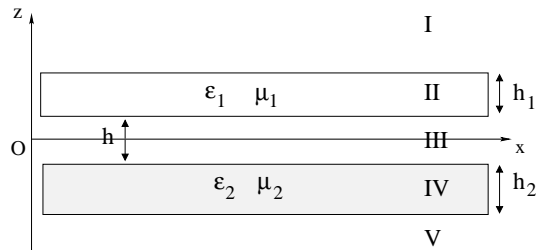
Figure 1: The two waveguides are surrounded by air and separated by a thickness h . The z = 0 plane is placed in the middle of the air layer (region III). The different regions are labelled using roman numerals.
