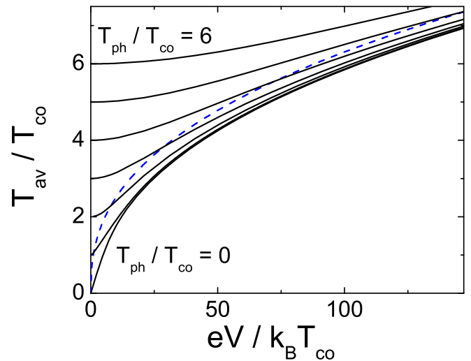
FIG. 3: (Color online) Average temperature T_{av} as a function of voltage V , for various temperatures T_{ph} , all in units of T_{co} = (\Sigma \Omega R e^2 / k_B^2)^{-1/3} . The value of T_{ph}/T_{co} is given by the intersection of the curves with the vertical axis. Blue dashed line is the reference temperature T_\Sigma .
