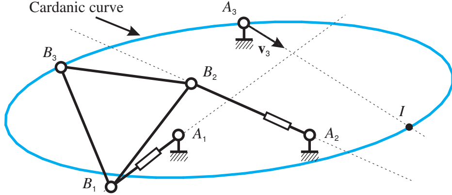
Figure 5. Cardanic curve of B_3 when B_1 and B_2 sliding along \mathbf{v}_1 and \mathbf{v}_2 , respectively
