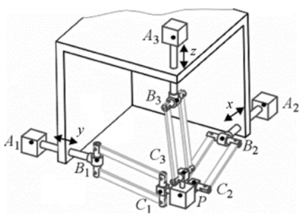
Fig. 1. Kinematic architecture of the Orthoglide
