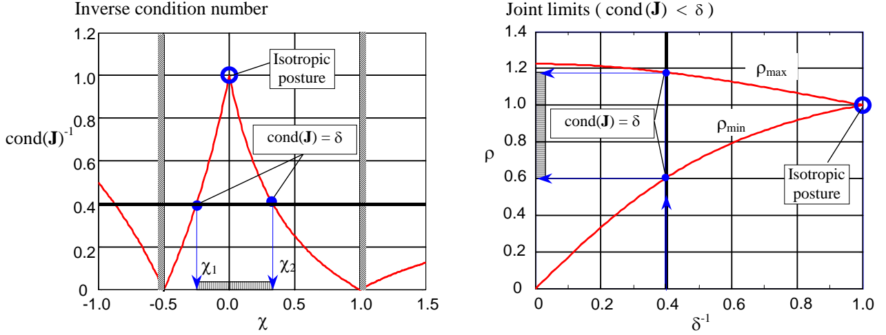
Fig. 6. Computing joint limits via the condition number.
