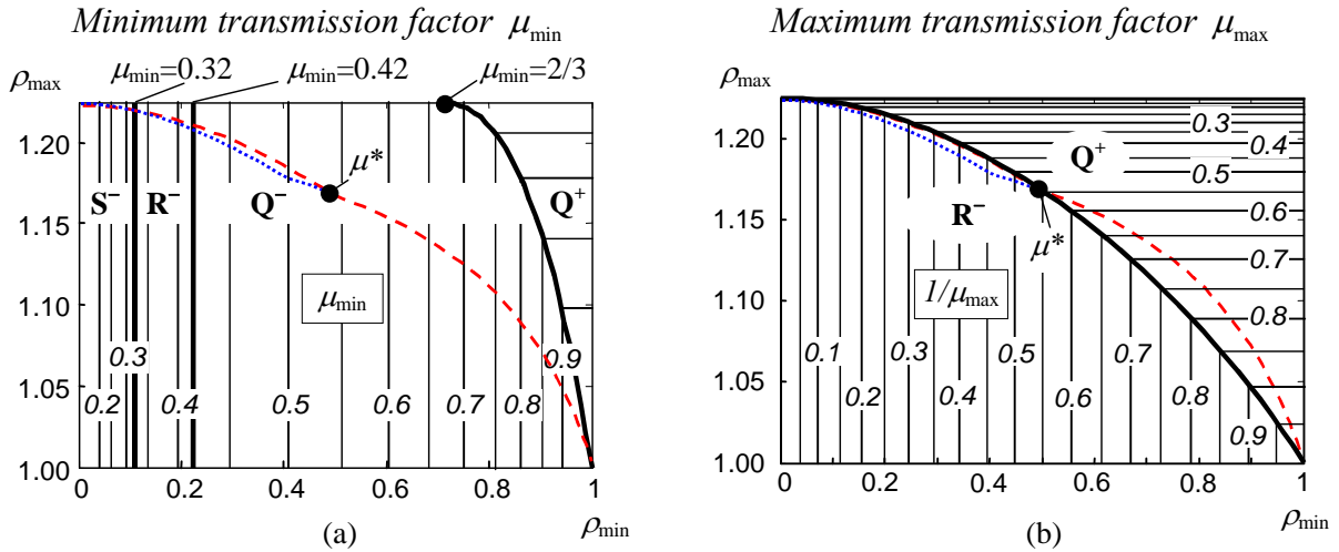
Fig. 9. Contour plots of the global transmission factors \mu_{\min} , \mu_{\max} on the plane \rho_{\min} \times \rho_{\max} (dashed/ dotted lines correspond to symmetrical constraints for W_\rho / Q -axis; \mu^* \approx 0.54 ).
