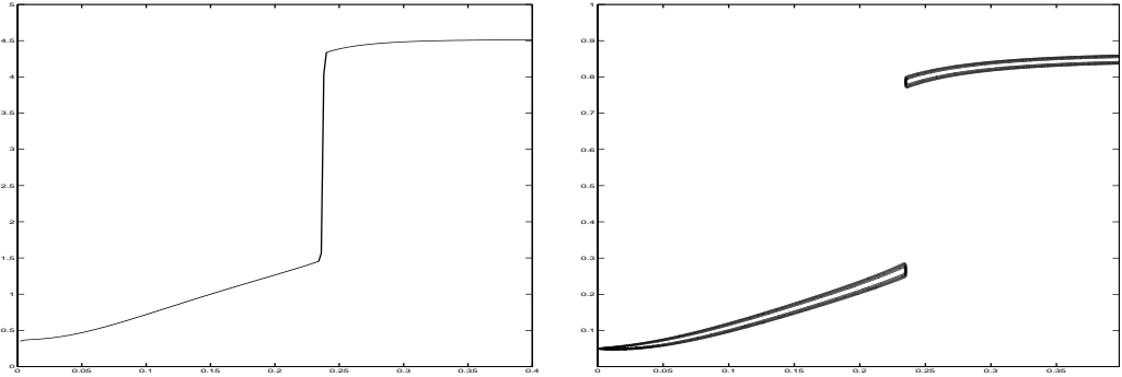
Figure 1: A NUMERICAL EXAMPLE OF DISCONTINUOUS SOLUTION IN EXAMPLE (38). THE ABCISSAE IS TIME. (LEFT) THE LAGRANGE MULTIPLIER \varrho(t) . (RIGHT) THE CONCENTRATION POINT \bar{x}(t) (IN FACT ISOVALUES OF THE DENSITY n_\varepsilon(t, x) ).
