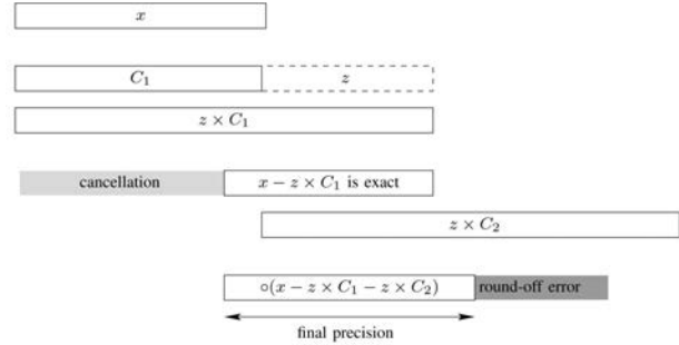
Fig. 3. Argument reduction with exact cancellation in an fma .
