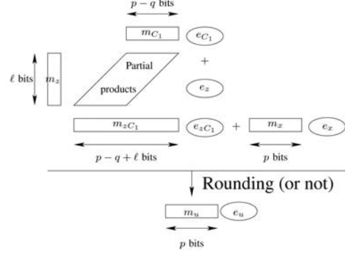
Fig. 6. \text{fma} used to create and cancel a higher precision virtual number.
